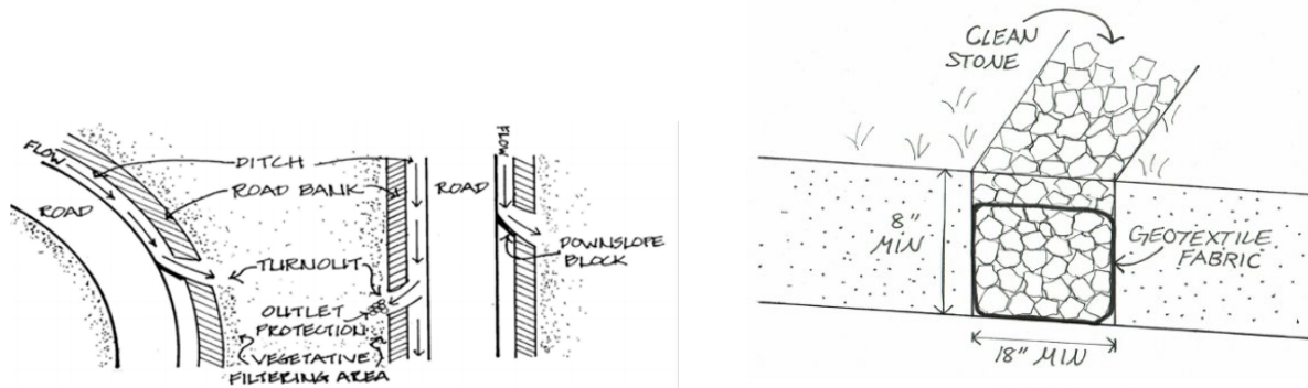
Figure 18: Infiltration Trench
